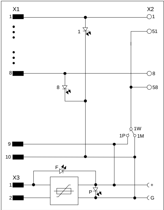
Fig. 8-7 Block diagram of interface module SB10
