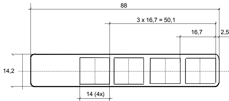
Fig. 10-4 Dimension drawing, labeling strips
