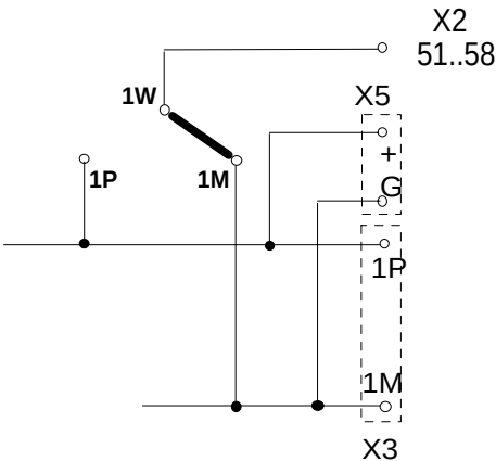
Fig. 8-5 Solder link to set the signal reference points
