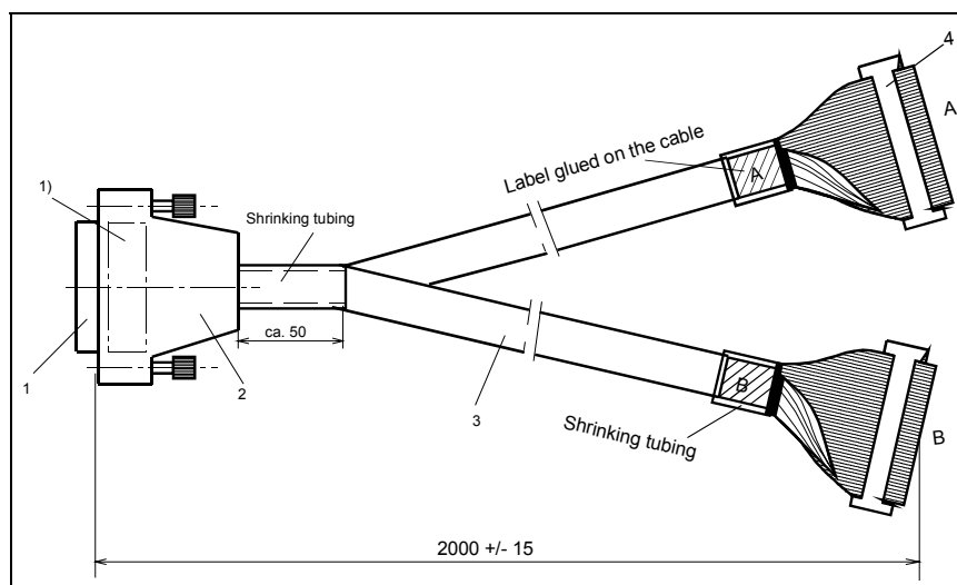
Fig. 9-2 Ribbon cable SC49
