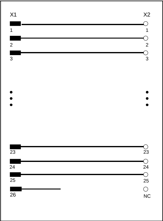
Fig. 8-17 Circuit diagram, SU10
