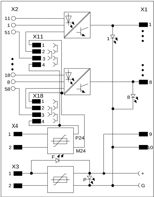
Fig. 8-12 Block diagram of interface module SB61
